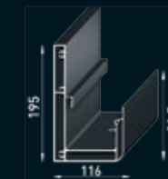
Integrated Beam
